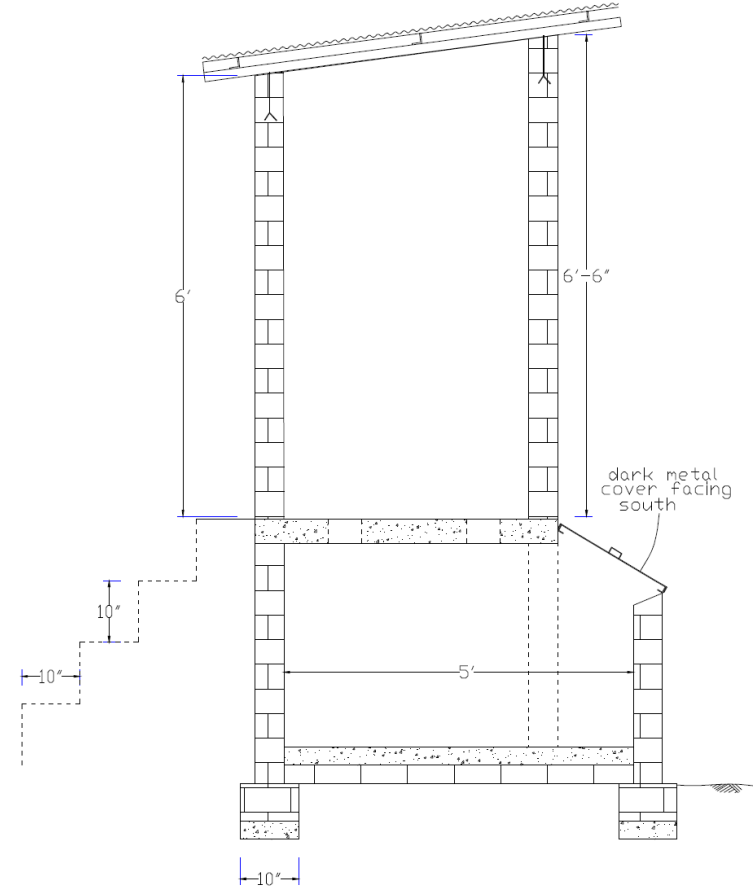
section-BB
