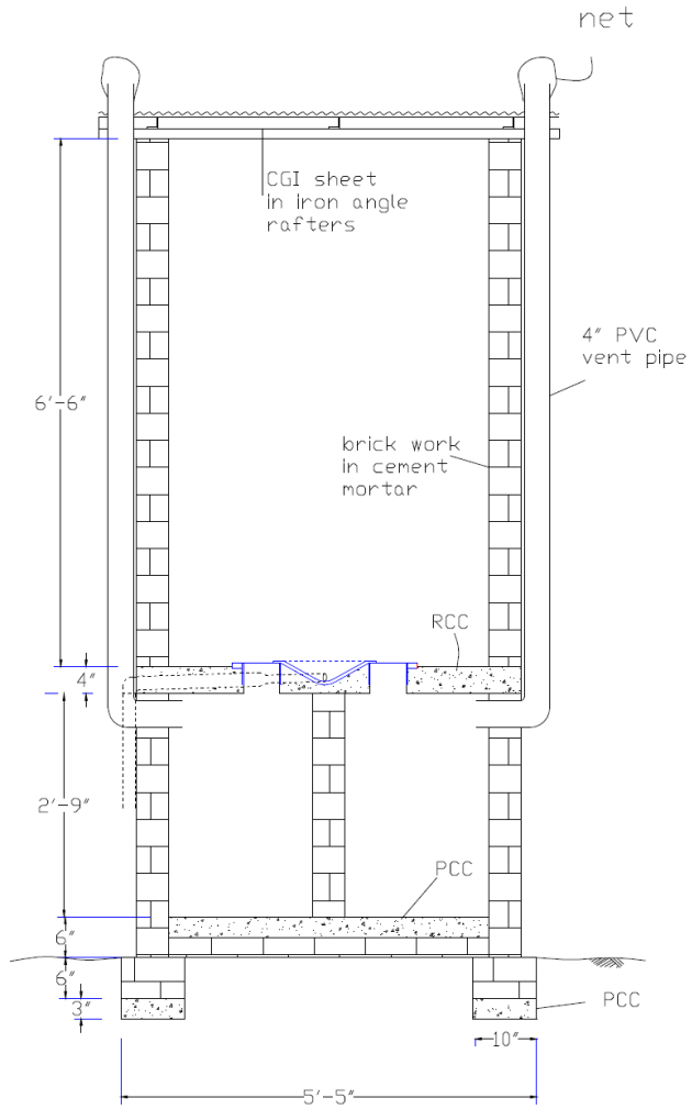
section-AA
