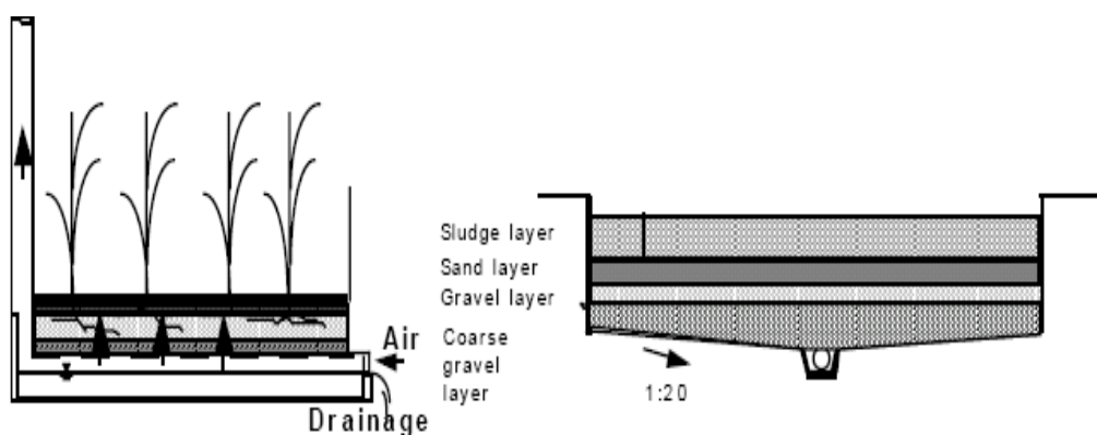
Figure 6.8 Schematic diagram of planted and unplanted sludge drying beds
