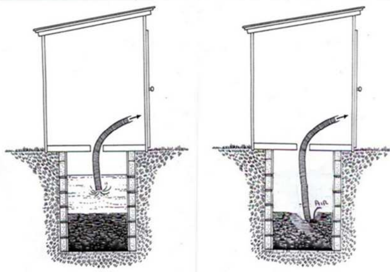
Figure 4.17 Air can enter the hose and break the flow when vacuuming dry sludge (Coffey)
