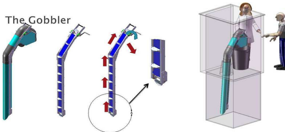
Figure 4.28 Initial design concept for the Gobbler
