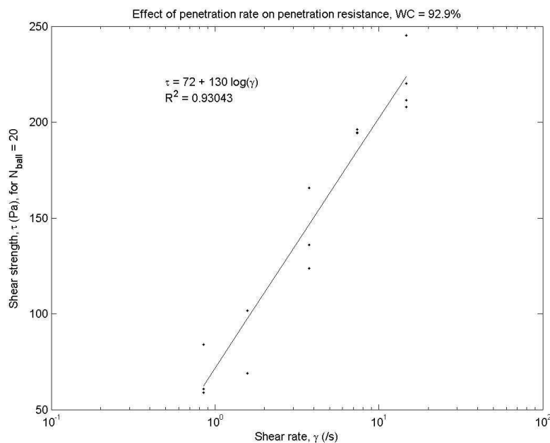
Figure 5: Semilog plot of ball penetrometer data
