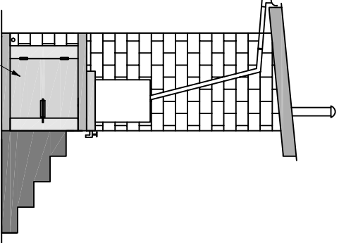
Superstructure with urinal
