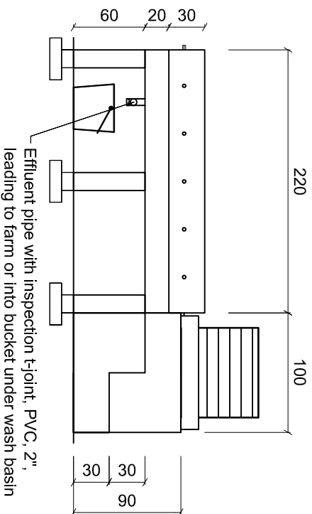
Front View Hand Wash Basin
