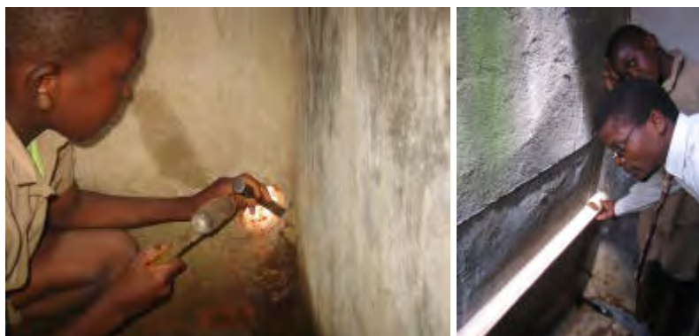
The PVC pipe is used as a urine collector and attached to the existing wall of the urinal. The pipe was 2.5m long made from 75mm PVC pipe. A section of 1.7m was cut out to form a channel in which the urine will flow. A hole is made in the external wall of the urinal and the pipe is placed along the existing urinal wall leading out through the wall to fit over the tank outside.
