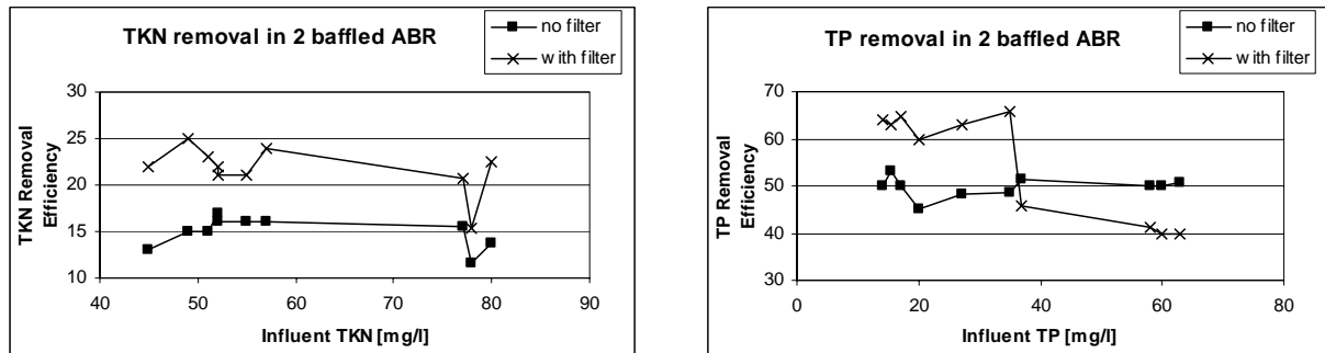
Figure 3: Removal efficiencies of nutrients (TKN and TP) in the 2 baffles ABRs
