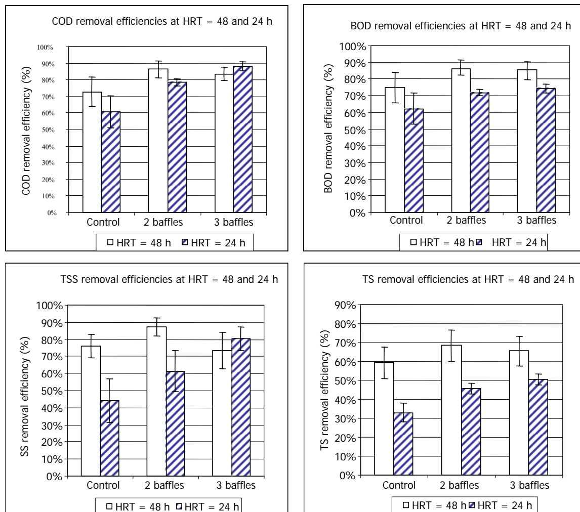
Figure 4: Removal efficiencies of COD, BOD, TS and SS in the different units at HRTs of 24 and 48 hours.
