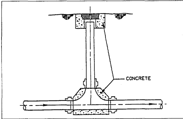
Figure 3.3. Inspection-cleanout (SABESP)
