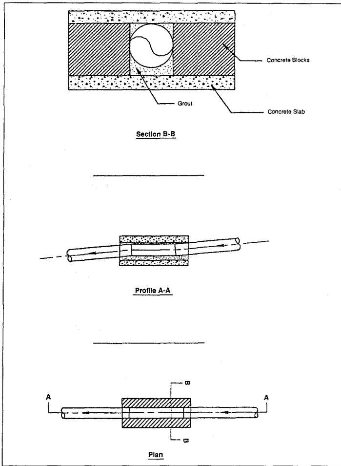
Figure 3.10b. Buried box for change in slope (SABESP)
