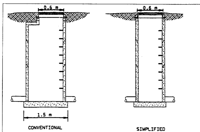
Figure 3.9a. Comparison of conventional and simplified manholes
