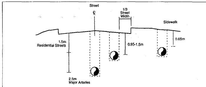
Figure 3.5. Minimum depths of sewers (SABESP)
