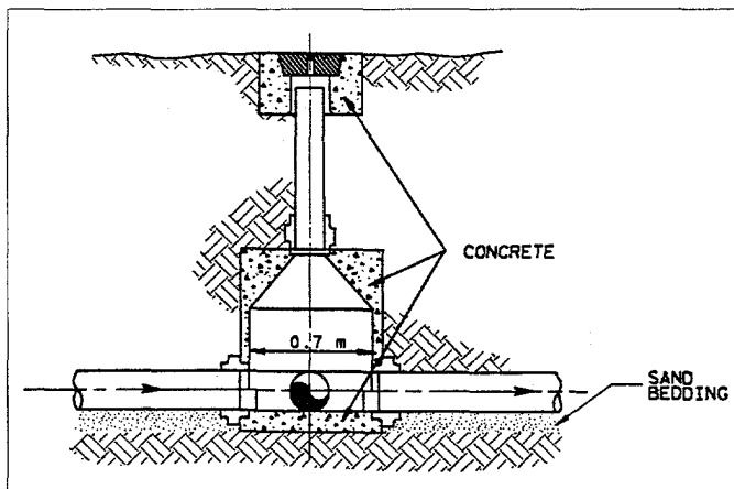
Figure 3.7. Junction inspection-cleanout
