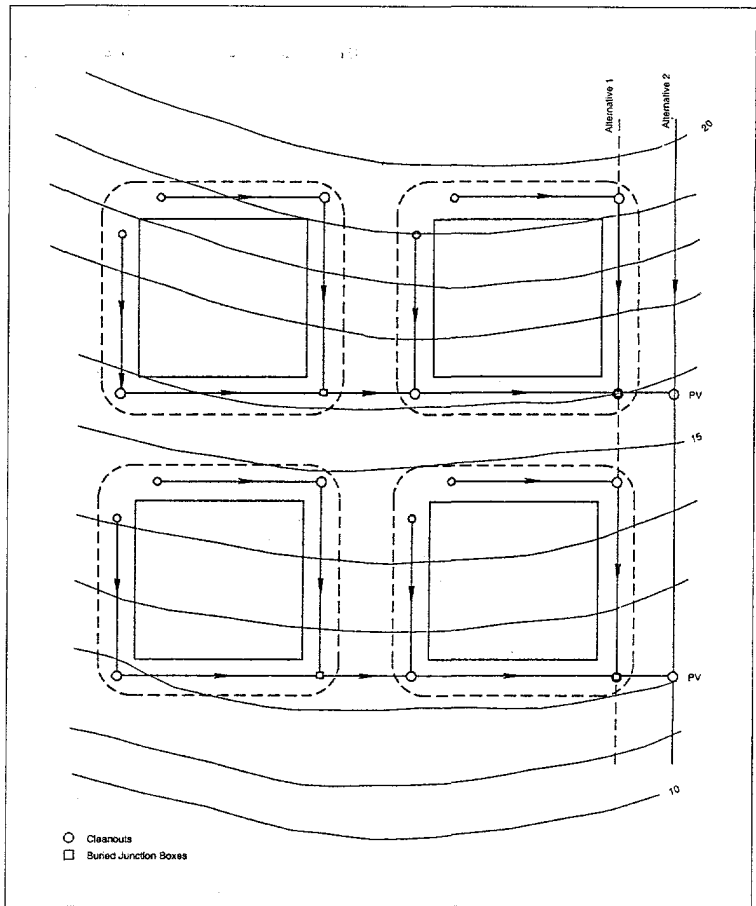
Figure 3.1. Typical layout of simplified sewer system (SABESP)
