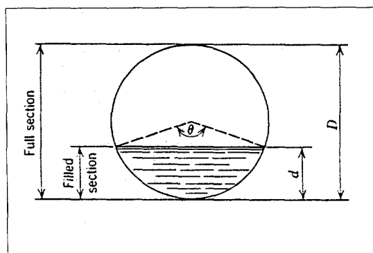
Figure A1. Elements of Circular Conduit
