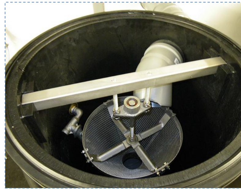
2 - Preceding screen (3 mm)
