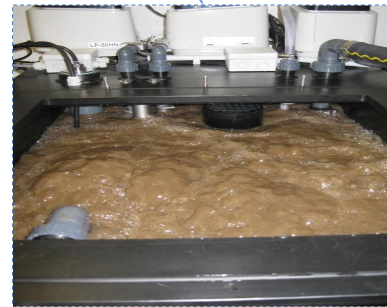
5 - Membrane bioreactor (MBR) Volume of tank 480 l
