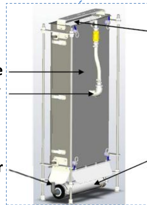
4 - Ultrafiltration module Plate membrane 3.5 m 2 / pore size 38 nm
