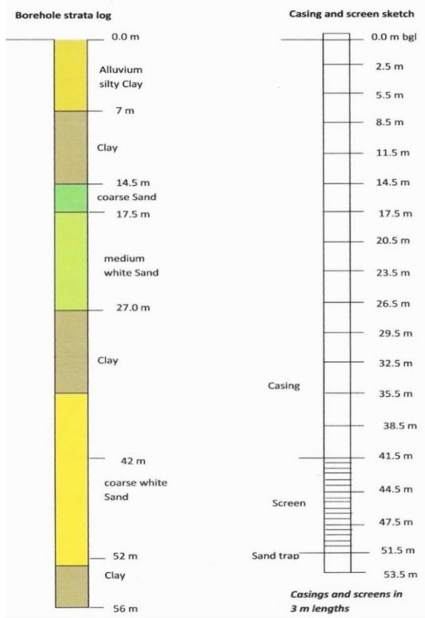
Figure 8: Casing and screen sketch in comparison to strata log
