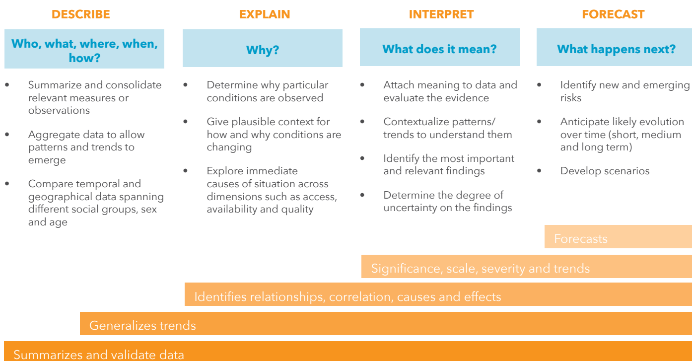
Figure 15: Analysis steps
