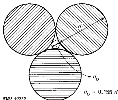
FIG. 3. RELATION BETWEEN GRAIN SIZE AND PORE SIZE
