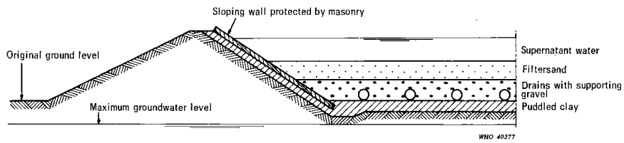
FIG. 12. SLOW SAND FILTER CONSTRUCTED OF MASONRY ON PUDDLED CLAY
