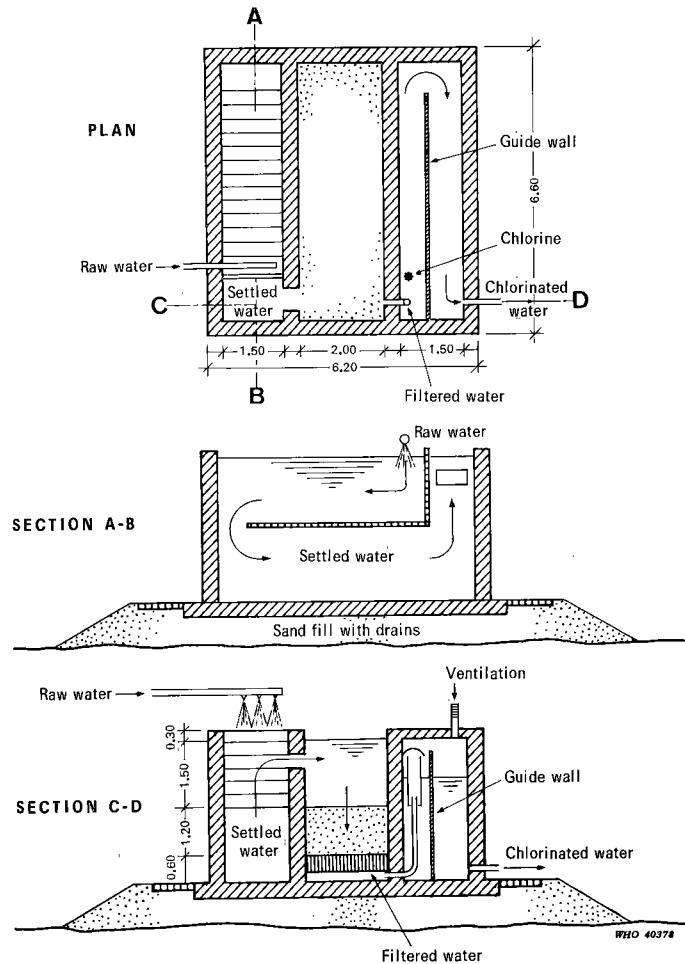
FIG. 16. VILLAGE WATER TREATMENT INSTALLATION, S URINAM
