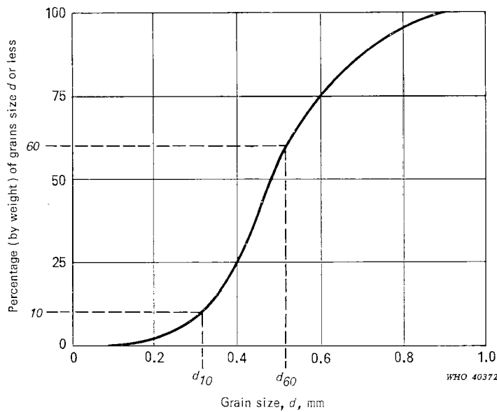
FIG. 5. SIEVE ANALYSIS
