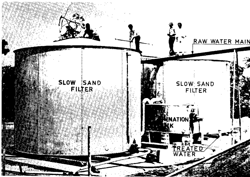
FIG. 14. CIRCULAR FILTERS FOR RURAL WATER SUPPLIES, SURINAM
