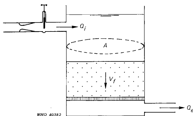
FIG. 20. UPSTREAM RATE CONTROL
