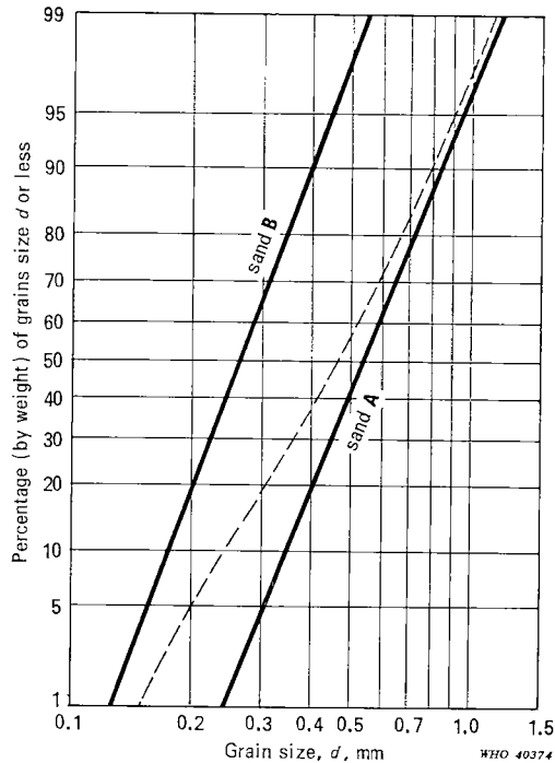
FIG. 8. COMBINATION OF TWO TYPES OF STOCK SAND
