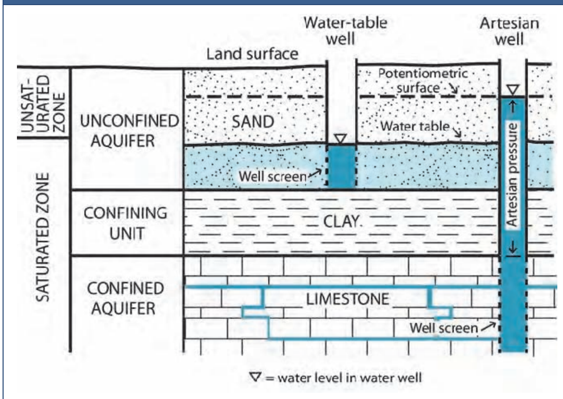
Figure 7.1: Well Hydrology
