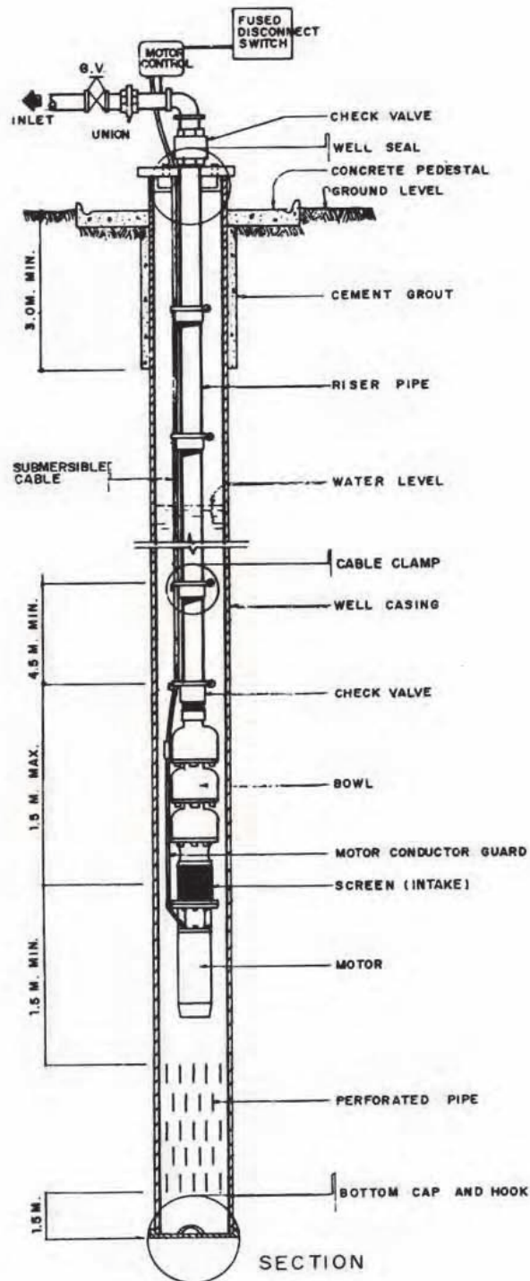
Figure 14.3: Submersible Pump
