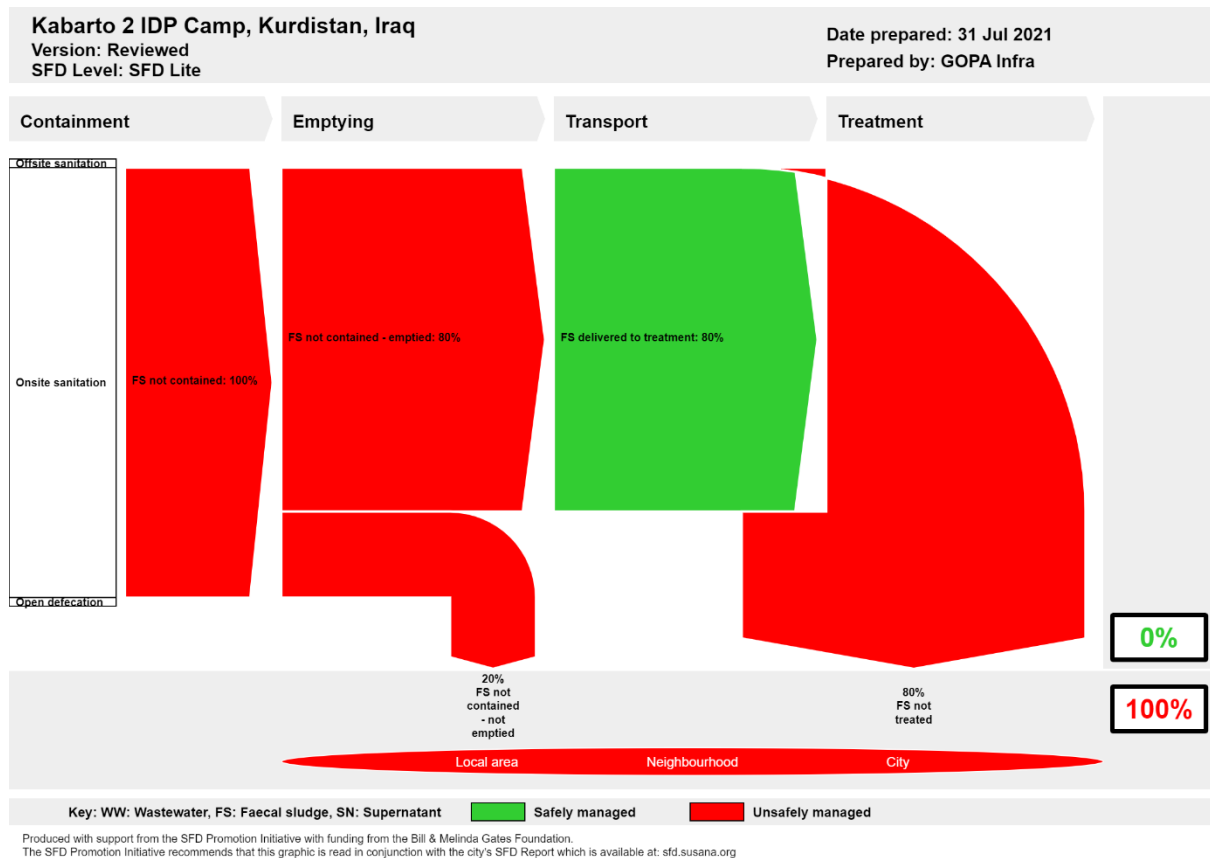
Figure 1 - SFD Graphic for Kabarto 2 IDP Camp
