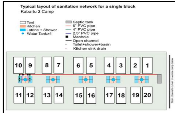
Figure 5 - Sanitation Collection System Kabarto 2 (Source: Duhok Governorate, 2021)
