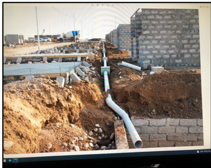
Figure 6 - Collection pipes from individual toilets (Source: Duhok Governorate, 2021)
