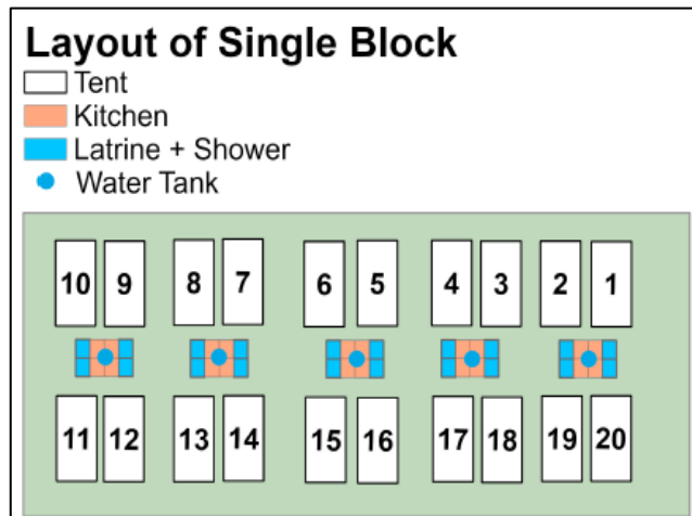
Figure 3 - Block Layout, Kabarto 2 (Source: CCCM Cluster Iraq, 2020)
