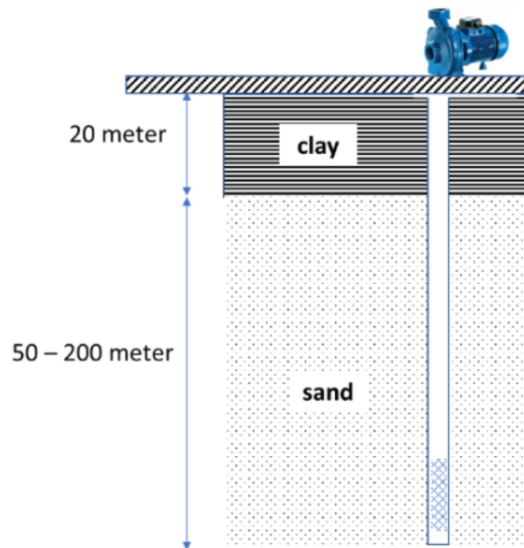
Figure 7: Soil profile Rajbari city and location of tube well screen.
