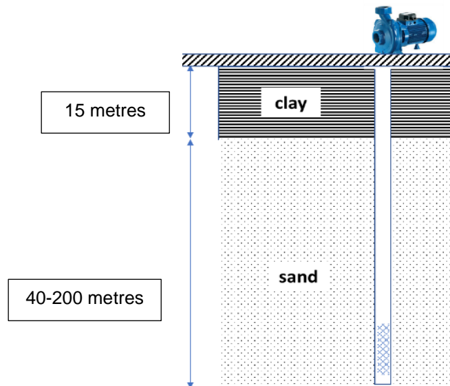
Figure 7: Soil profile in Bogra district and location of tube well screen.
