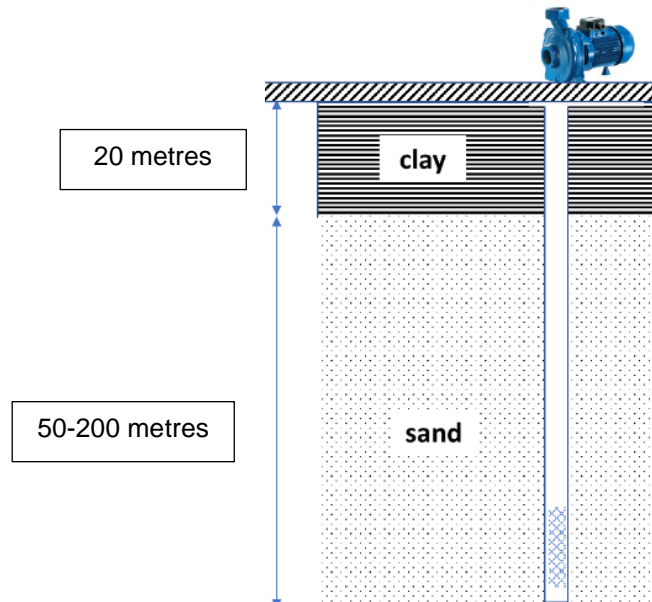
Figure 5: Soil profile in Galachipa Upazila and location of tube well screen.
