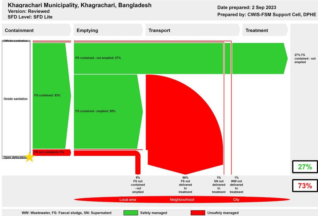
Figure 7: SFD Graphic for Khagrachari Municipality.
