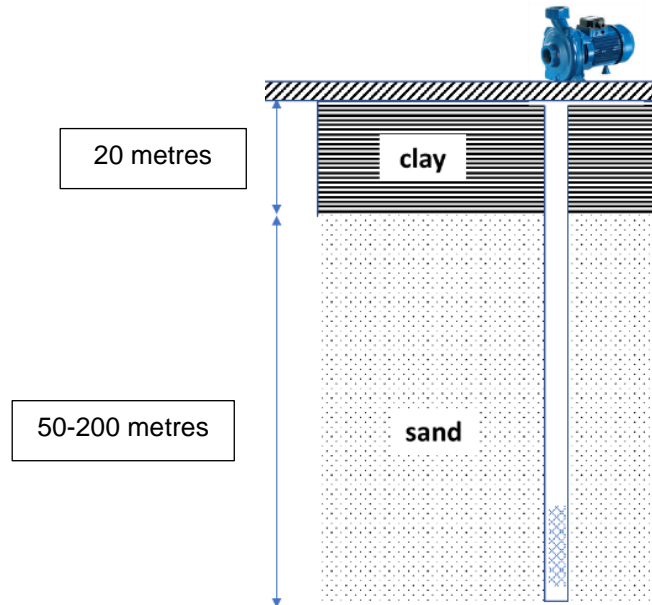
Figure 5: Soil profile in Khagrachari district and location of tubewell screen.
