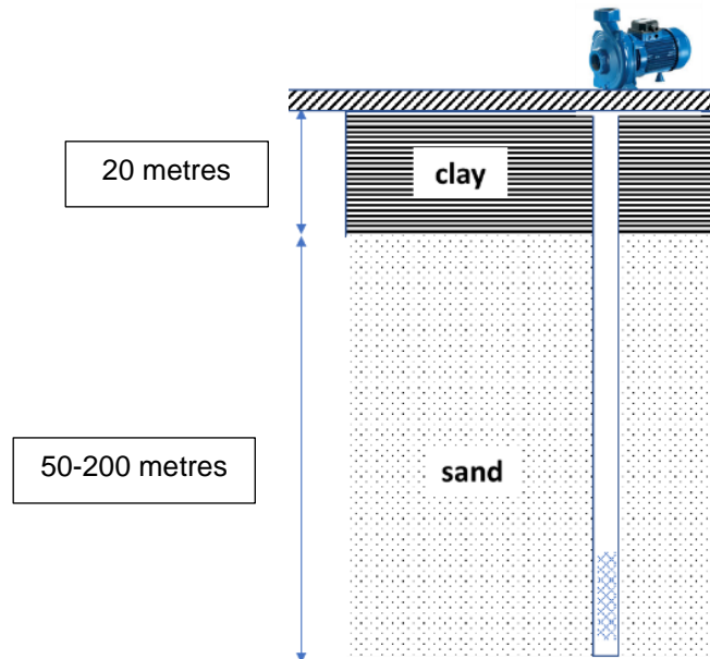
Figure 5: Soil profile in Habiganj district and location of tubewell screen.
