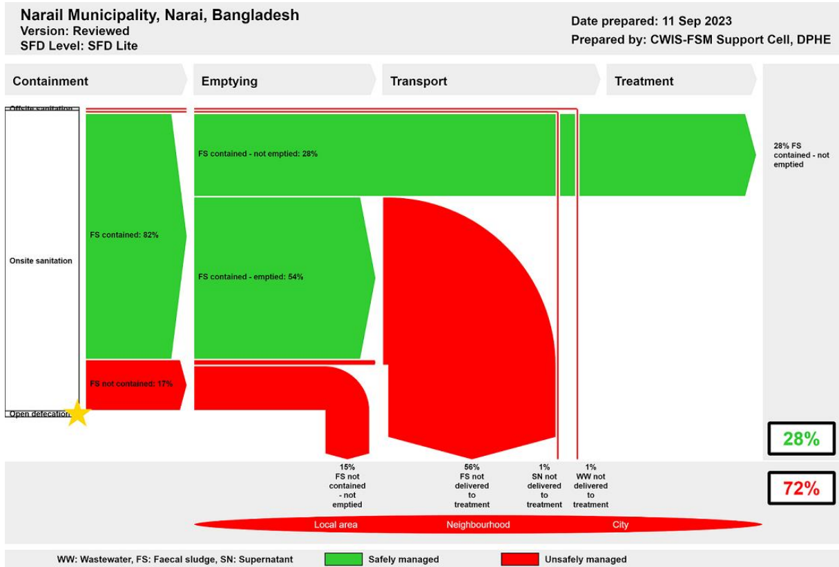
Figure 7: SFD Graphic for Narail Municipality.
