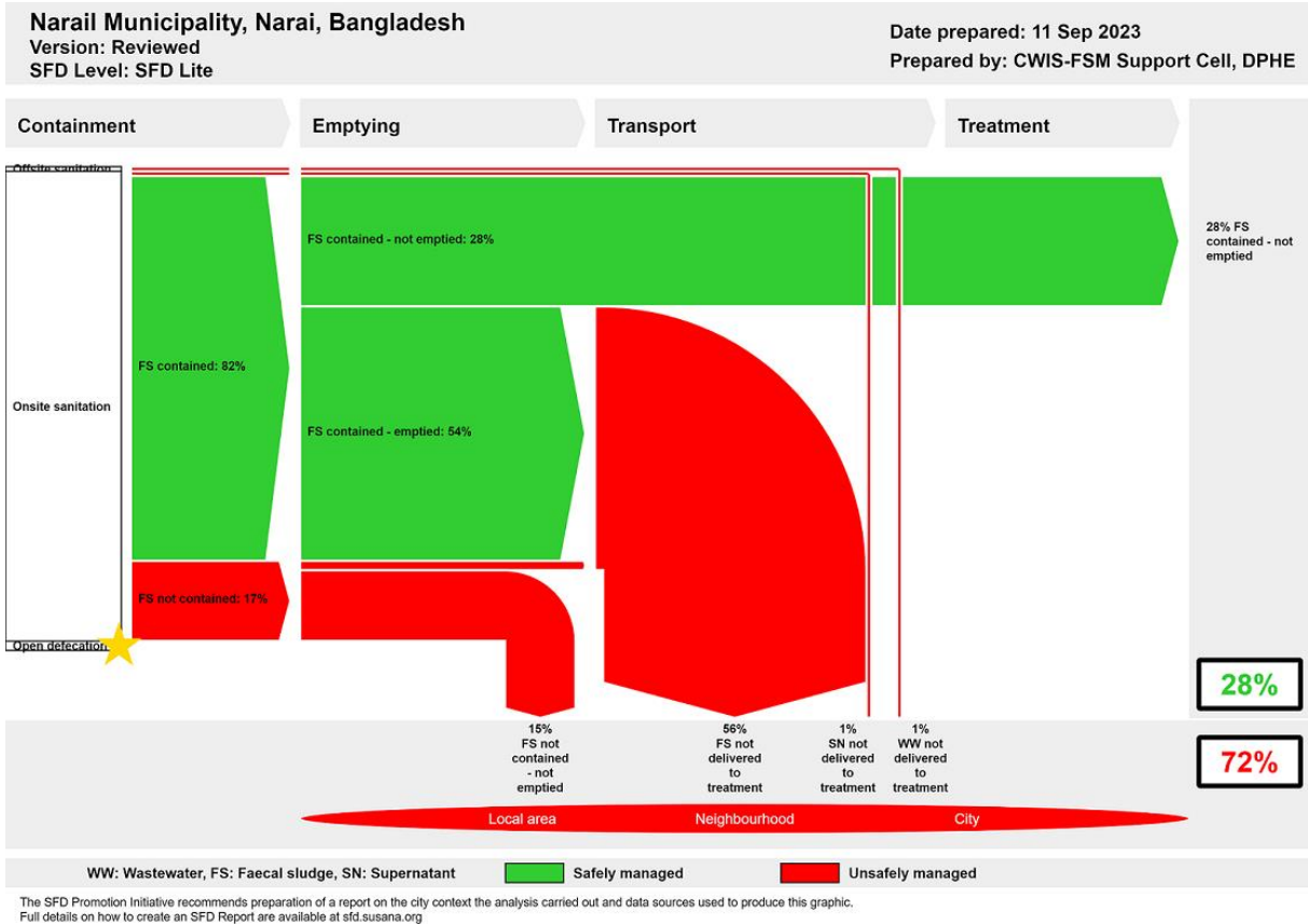
Figure 1: SFD Graphic for Narail Municipality.
