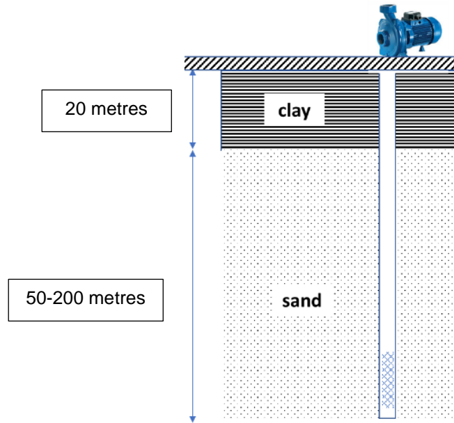
Figure 5: Soil profile in Narail district and location of tubewell screen.
