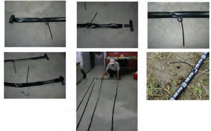
Figure 20. Laying out drip lines with inserted drippers (emitters).
