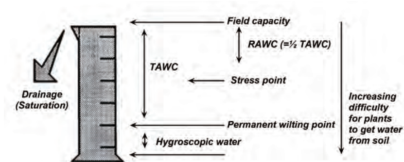
Figure 31. Soil water holding characteristics and terms. (Luke, 2006)
