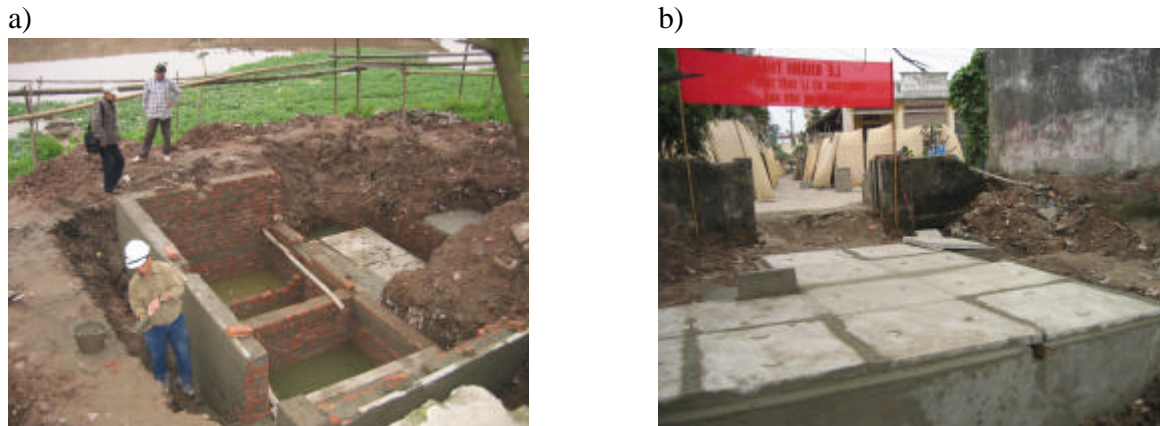
Figure 4. Baffled Septic Tank P-20 serving 20 households in Huu Hoa Commune: a) during construction; b) construction completed. (photo by Nguyen V. A., 2006)
