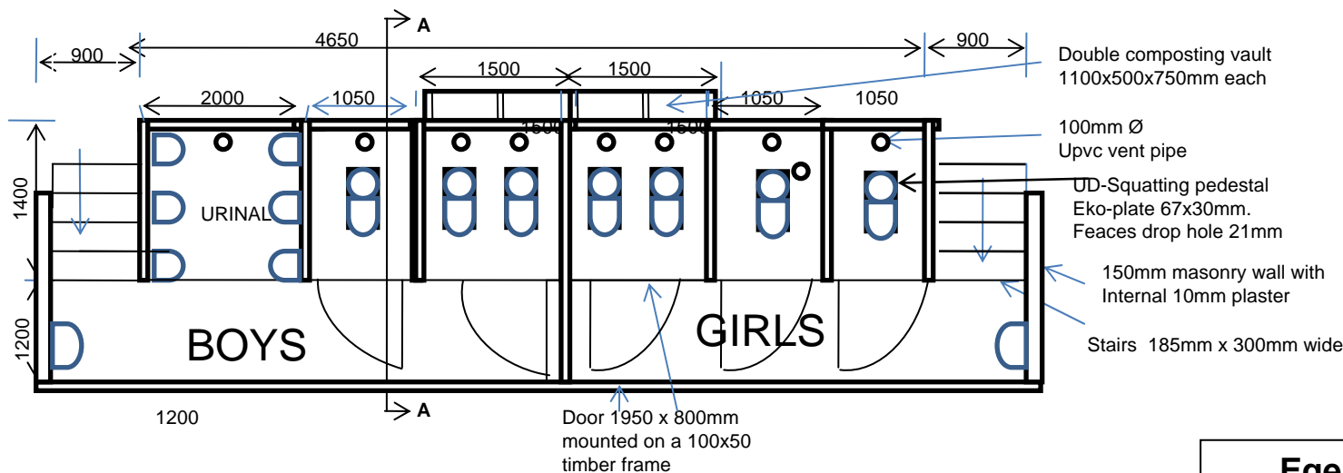
Ground Plan
