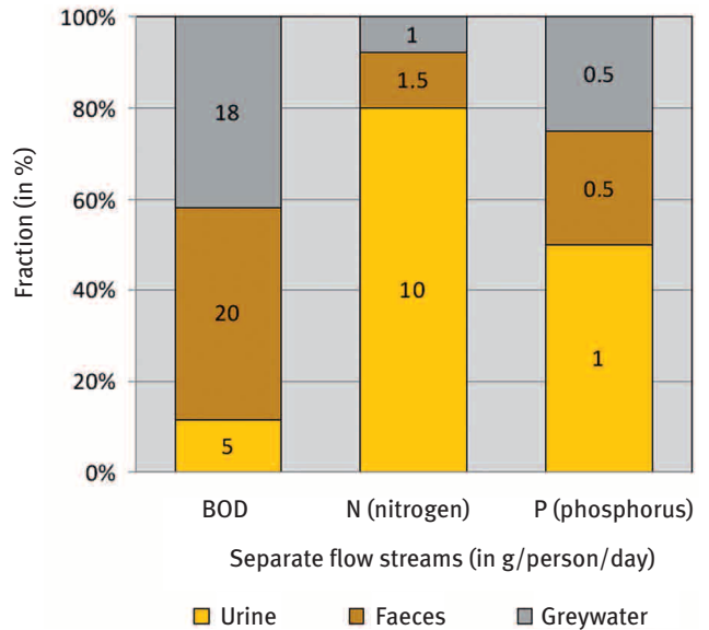
Top chart: Content of the different domestic wastewater streams (urine, faeces, greywater) in percentages and absolute values (BOD is biological oxygen demand).
