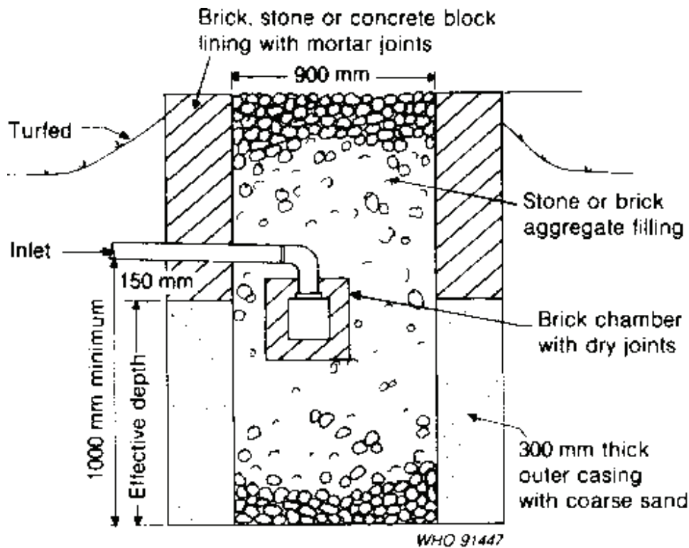
Fig. 6.28. Unlined oakpit
