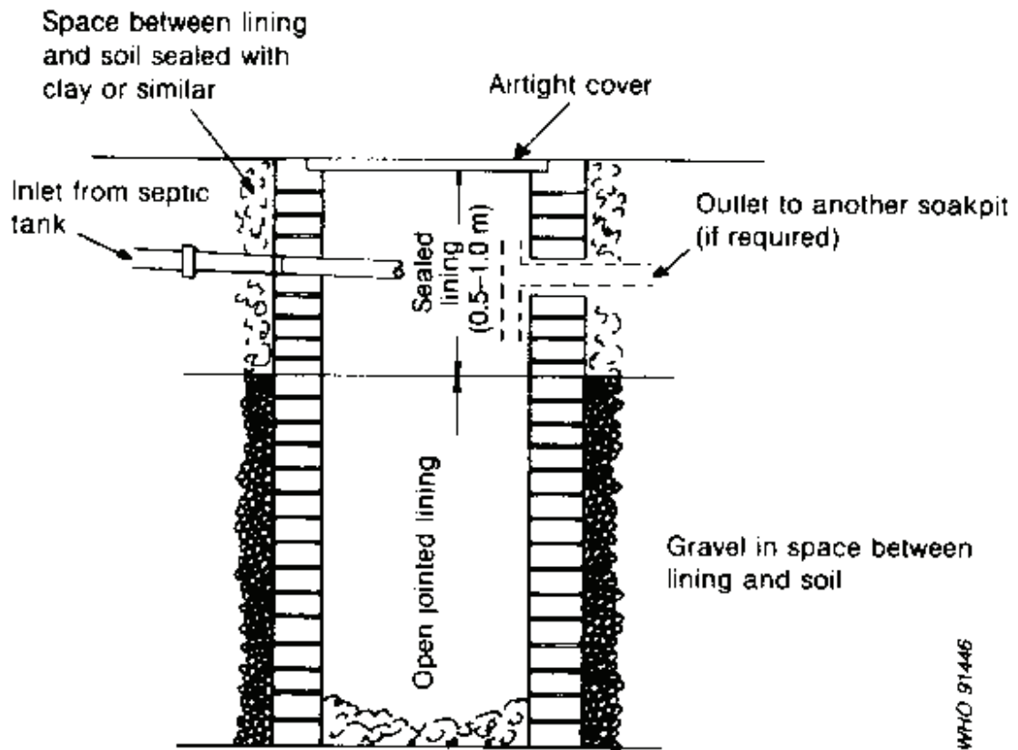
Fig. 6.27. Lined soakpit
