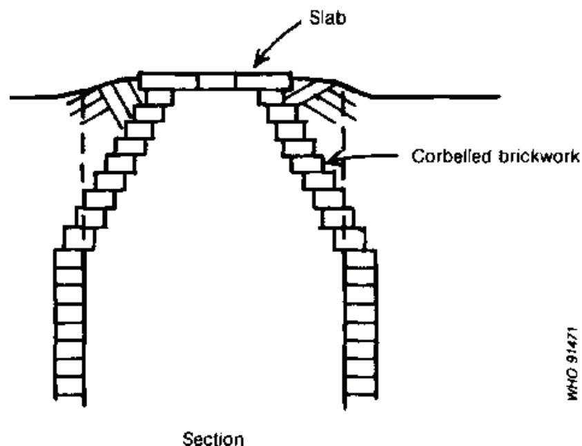
Fig. 7.11. Minimizing the span of the slab
