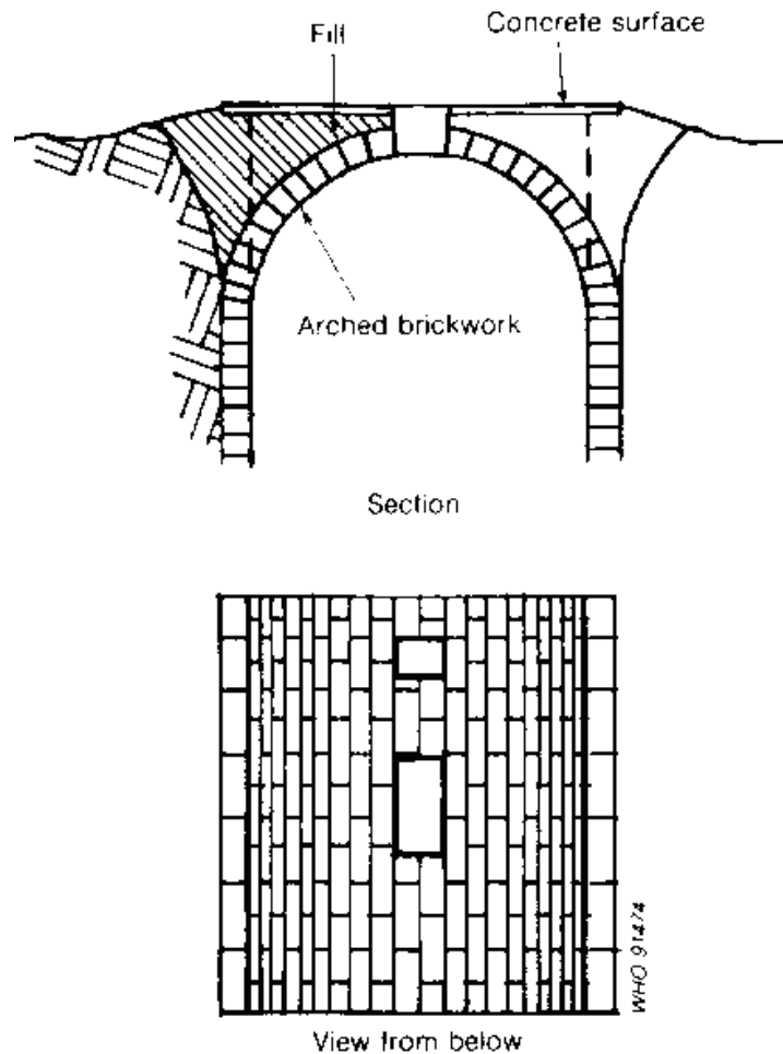
Fig. 7.14. Arched brickwork lining and support
