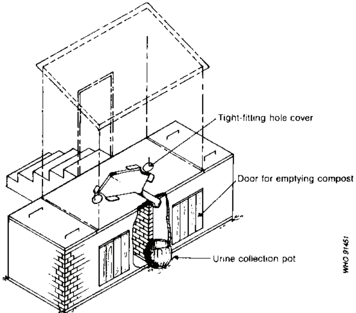
Fig. 6.32. Double-vault latrine
