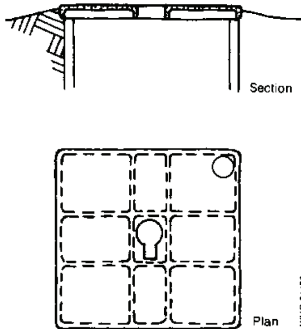
Fig. 7.16. Ferrocement slab
