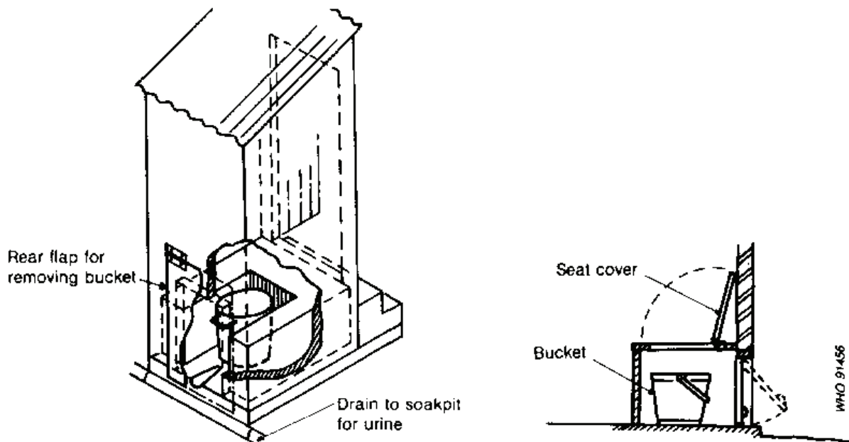
Fig. 6.37. Bucket latrine
