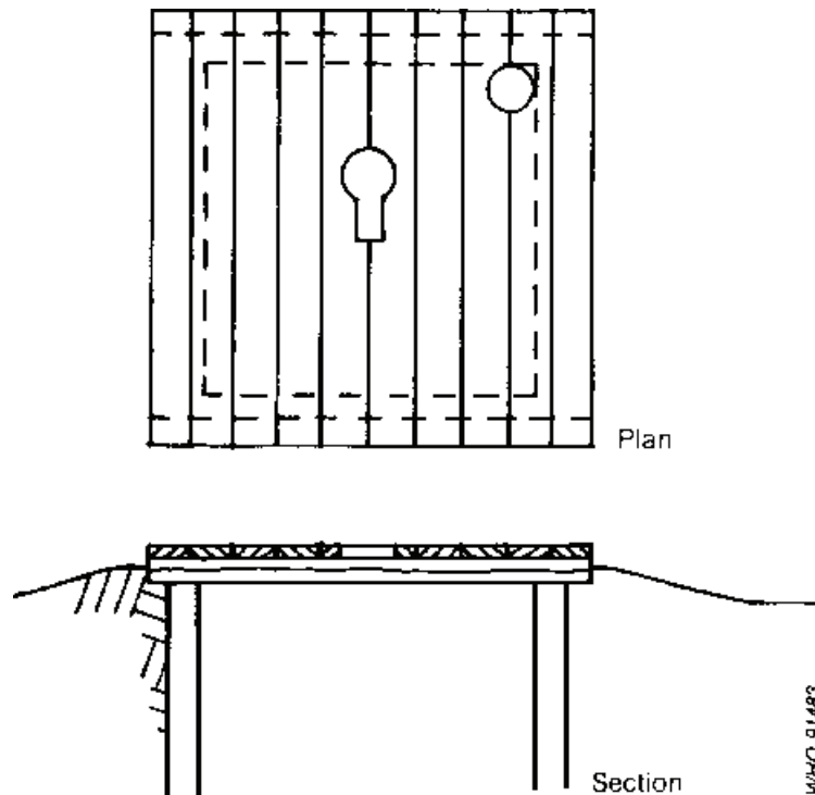
Fig. 7.23. Sawn timber slab
