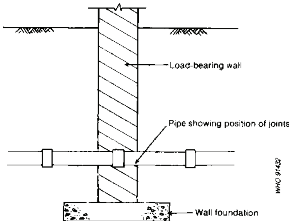
Fig. 6.13. Pipe fixed in place through a wall
