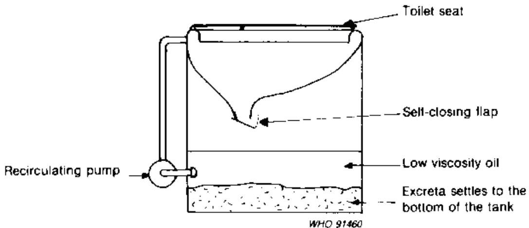
Fig. 6.41. Recirculating oil toilet
