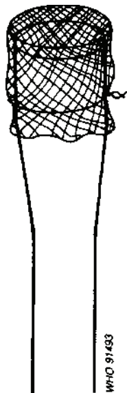
Fig. 7.33. Belled vent with fly screen
