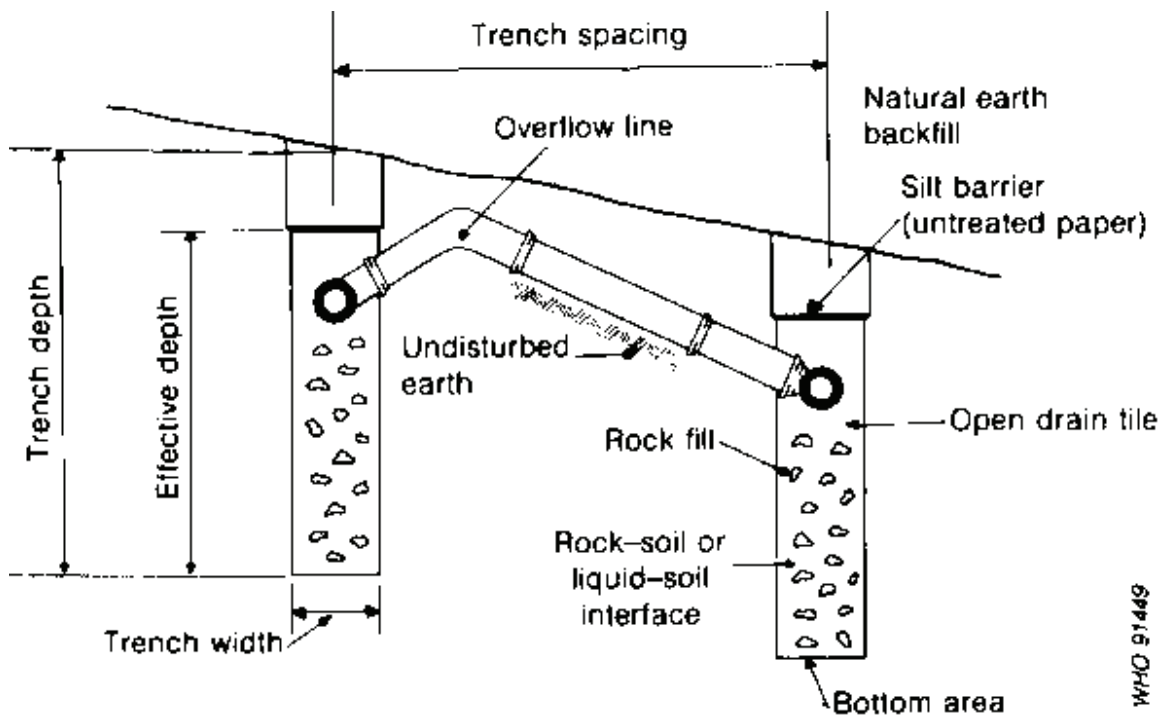
Fig. 6.30. Drainage trench
