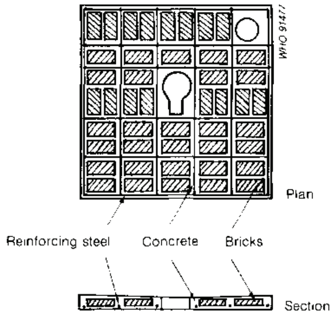
Fig. 7.17. Reinforced brickwork slab
