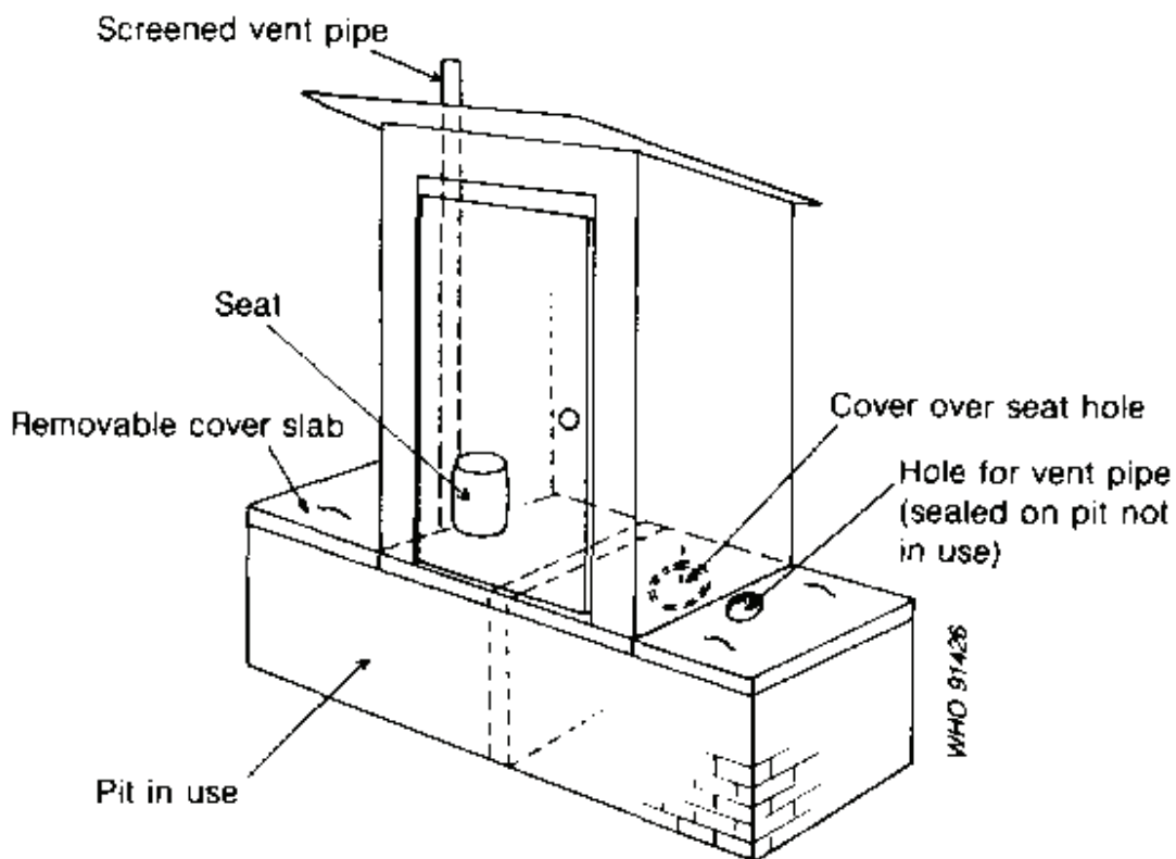
Fin. 6.7. Double-nit VIP latrine
