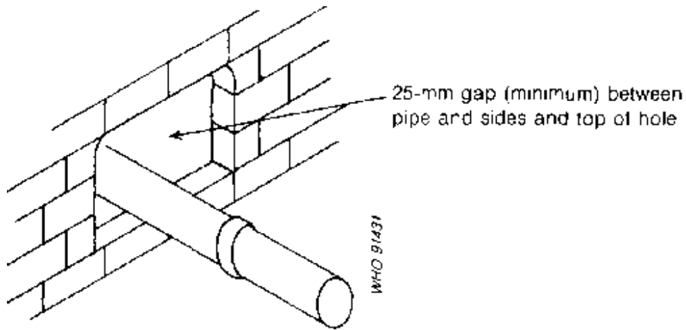
Fig. 6.13. Pipe fixed in place through a wall
