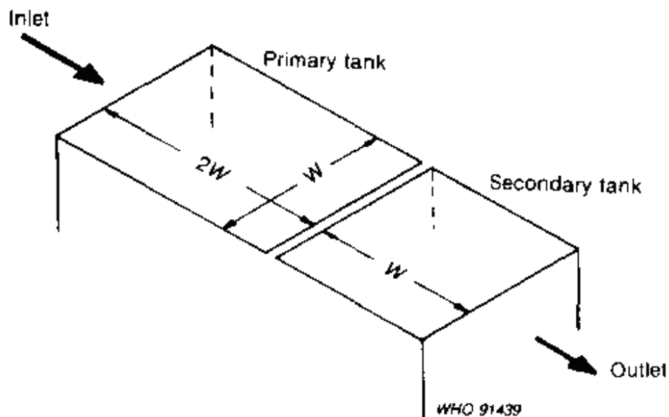
Fig. 6.20. Tank dimensions
