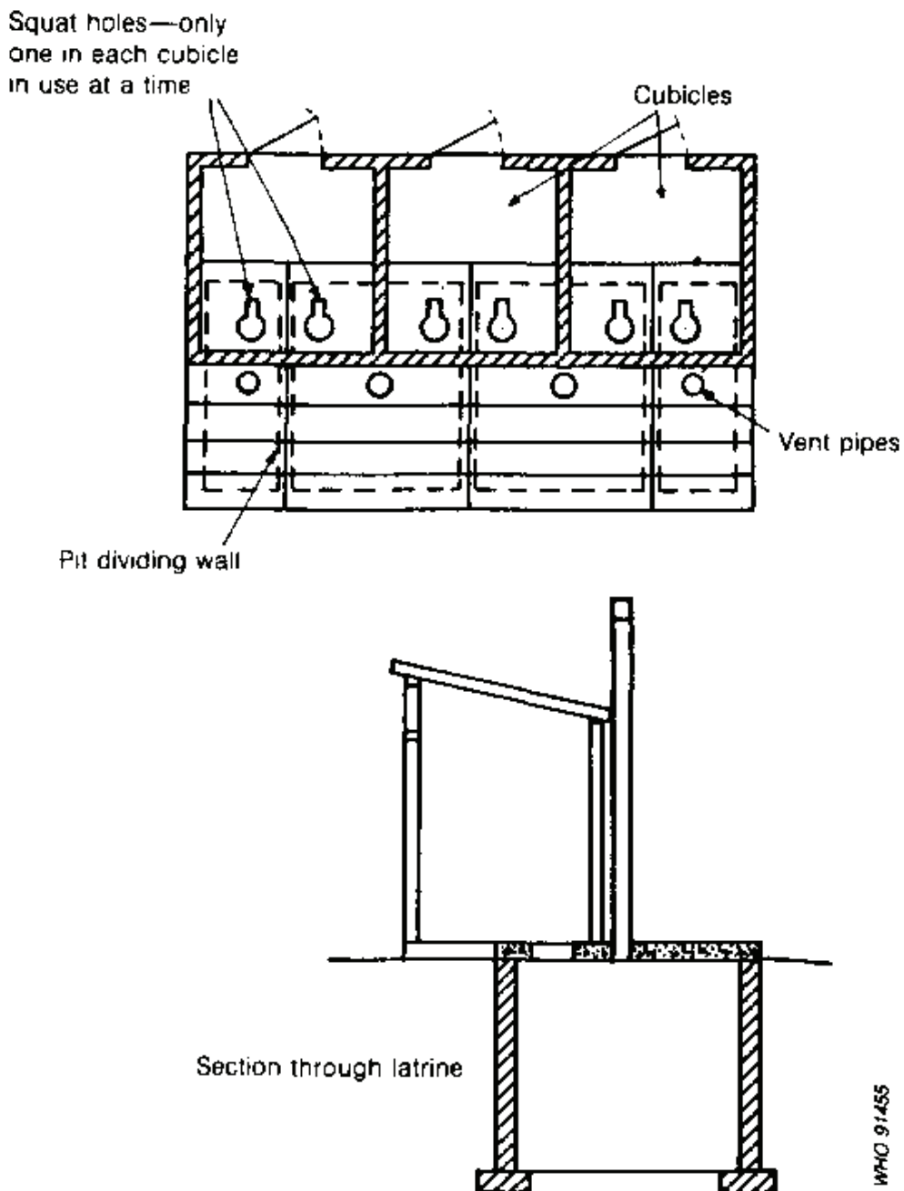
Fig. 6.36. Multiple double-pit VIP latrine
