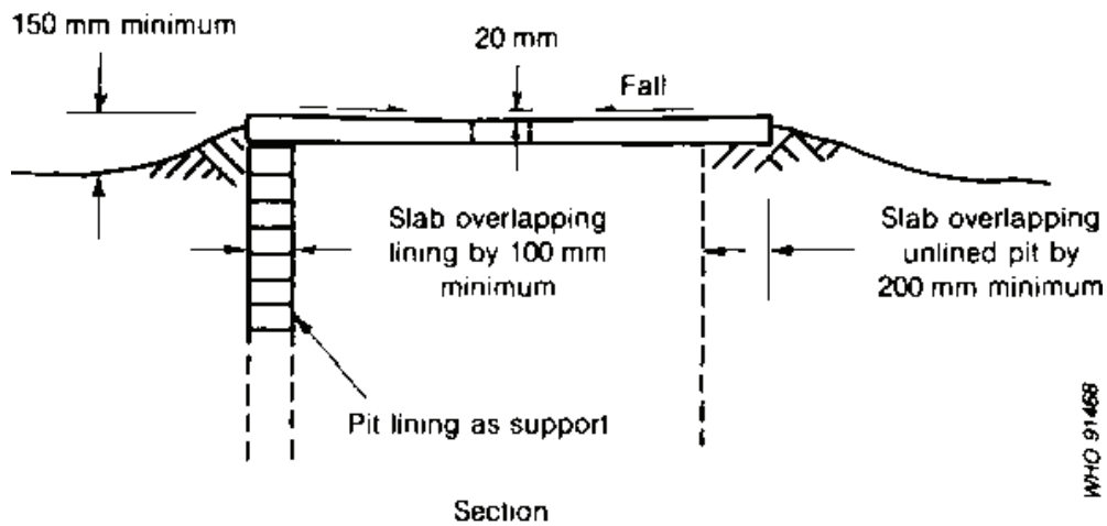
Fig. 7.8. Requirements of slabs
