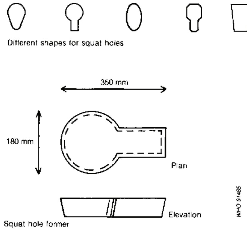
Fig. 7.25. Squat hole shapes and former
