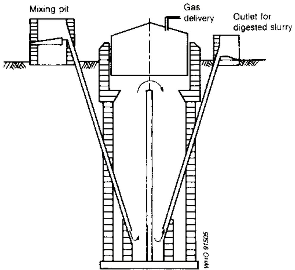
Fig. A1.5. Biogas plant with floating dome
