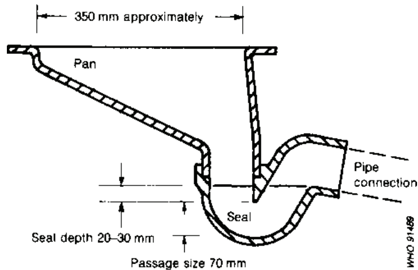
Fig. 7.29. Pan and seal for offset pour-flush latrine
