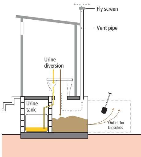
Figure 3: Design of EcoSan toilets
