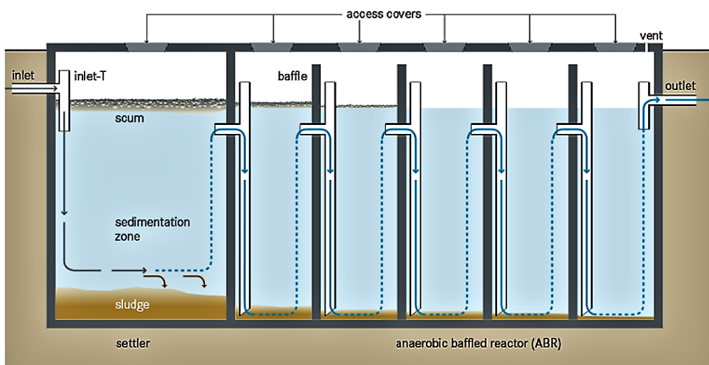
Figure 9: Design of anaerobic baffle reactor
