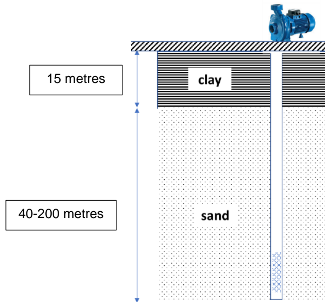
Figure 7: Soil profile in Lalmonirhat district and location of tube well screen.
