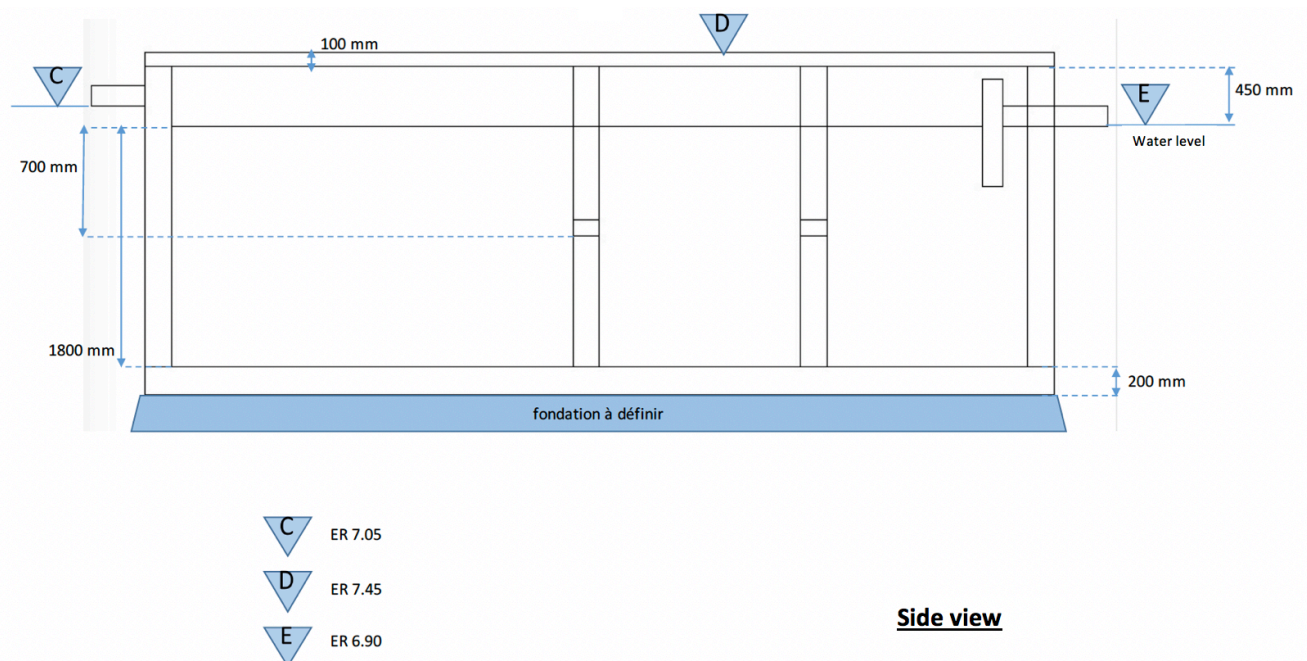
Figure 29: detailed drawing of the septic tank, top and side view
