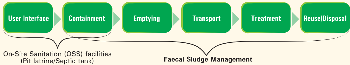
Figure 1: Components of faecal sludge management system
