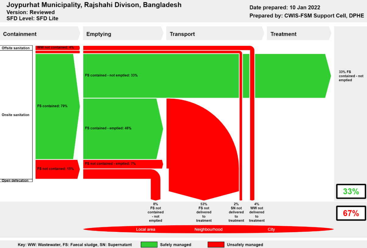
Figure 1: SFD Graphic for Joypurhat municipality.
