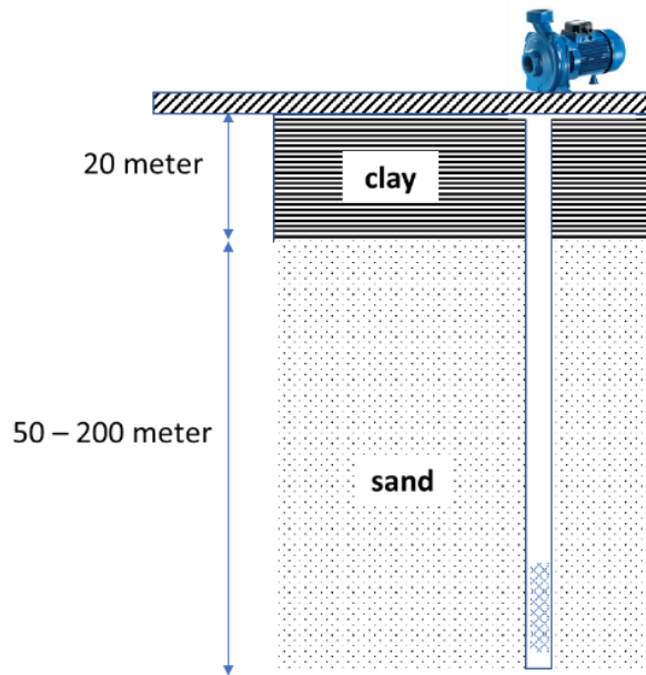
Figure 6: Soil profile Thakurgaon city and location of tube well screen.
