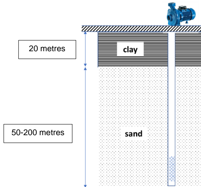
Figure 5: Soil profile in Gopalganj district and location of tubewell screen.
