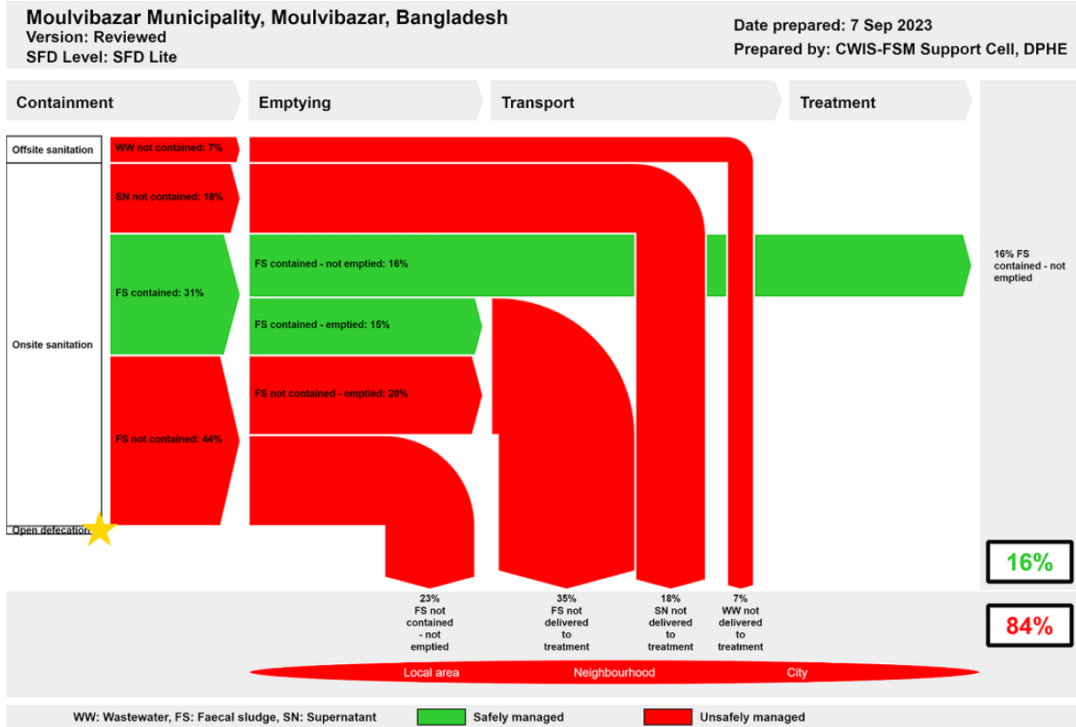
Figure 7: SFD Graphic for Moulvibazar Municipality.
