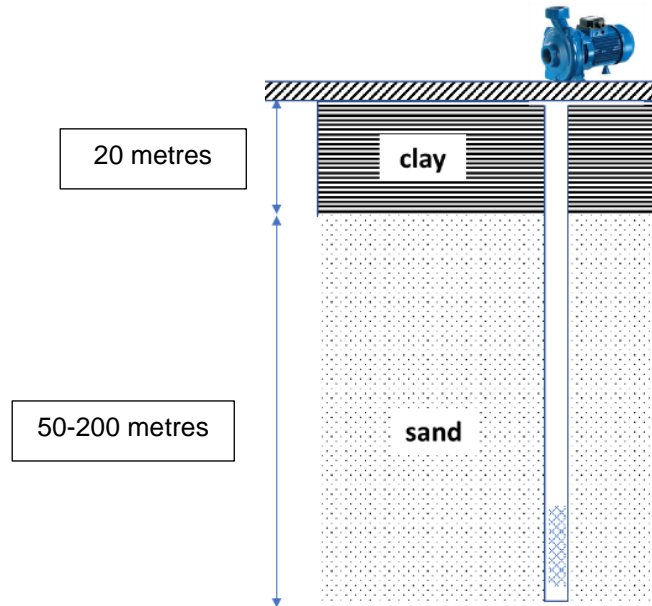
Figure 5: Soil profile in Moulvibazar district and location of tubewell screen.
