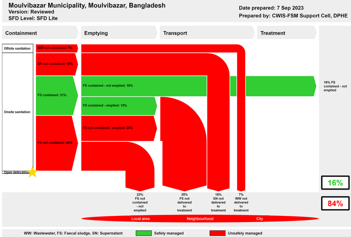
Figure 1: SFD Graphic for Moulvibazar Municipality.
