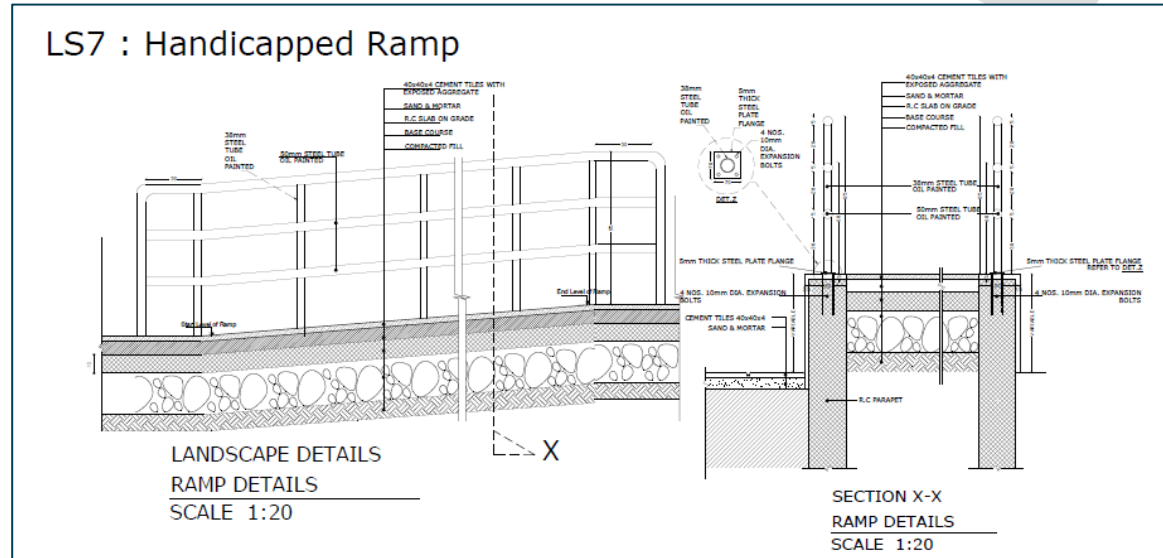
Figure 4&5: Ramp with appropriate surface and slope (source internal from S4M in Jordan in 2022)
