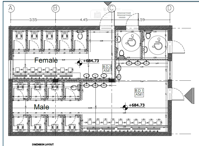
Figure 2&3: WASH facilities with ramp for disabled visitors and exemplary sanitary unit layout (source internal from SAM in Jordan in 2022)
