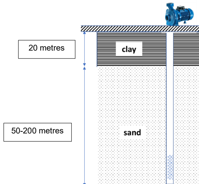
Figure 5: Soil profile in Sreemangal Upazila and location of tubewell screen.
