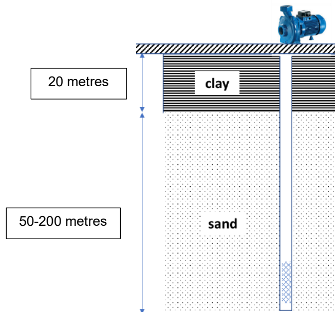
Figure 5: Soil profile in Manohardi Upazila and location of tubewell screen.
