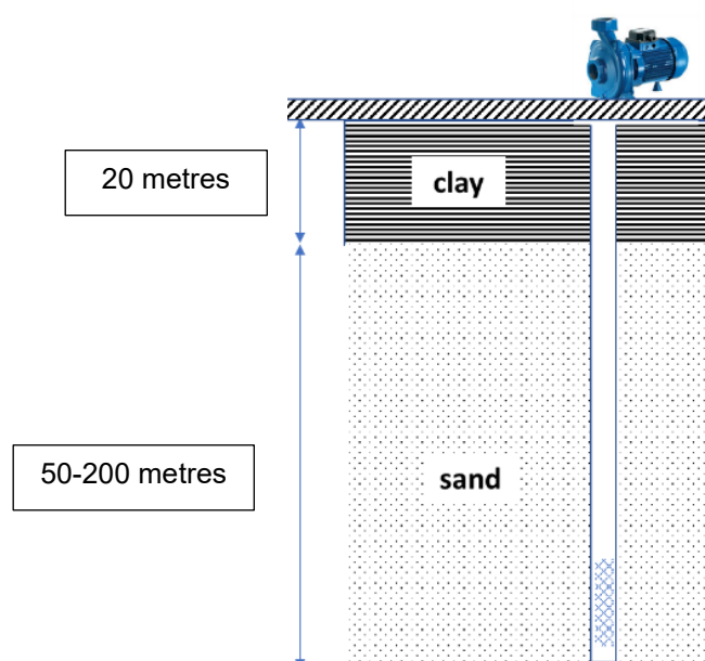
Figure 5: Soil profile in Karimganj Upazila and location of tubewell screen.
